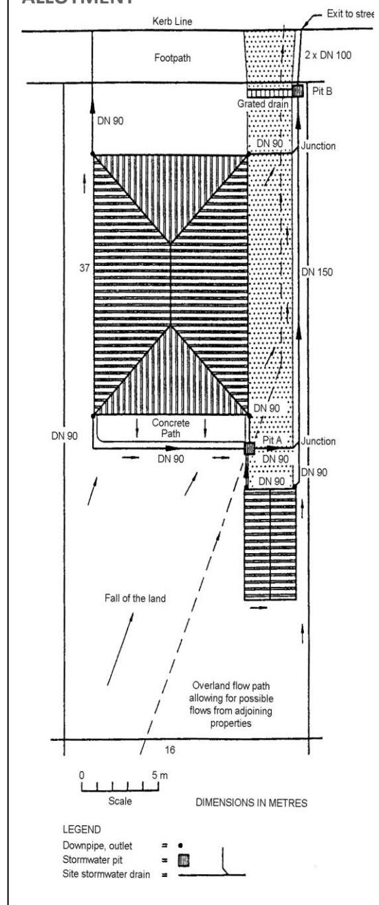
FIGURE 2 – SOLUTION TO STORMWATER DRAINAGE ON URBAN ALLOTMENT
