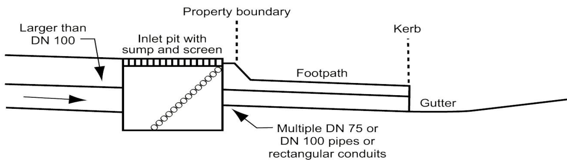
FIGURE 8.1 TYPICAL ARRANGEMENT OF INLET PIT AND FOOTPATH CROSSING
