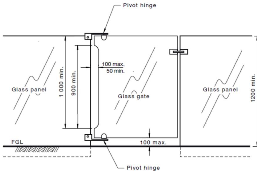
Figure 6: Glass gate with pivot hinges, referenced from AS1926.1, Figure 2.4 Reproduced with permission of Standards Australia Limited. Copyright in AS/NZS:2012 vests in Standards Australia Limited and Standards New Zealand.
