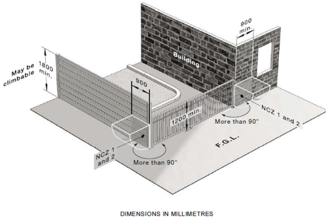
Figure 5: Intersecting internal barriers, referenced from AS1926.1, Figure 2.3 Reproduced with permission of Standards Australia Limited. Copyright in AS/NZS:2012 vests in Standards Australia Limited and Standards New Zealand.
