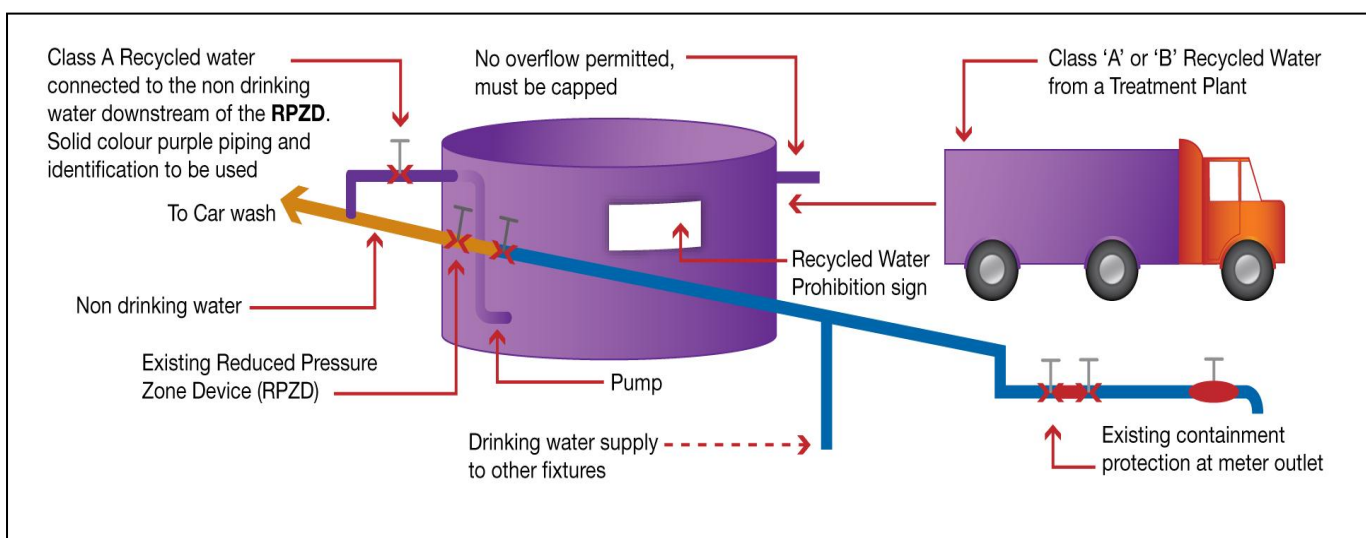
FIGURE 2 - ON SITE TANKER FILLING OR RECYCLED WATER FOR COMMERCIAL CAR WASHING
