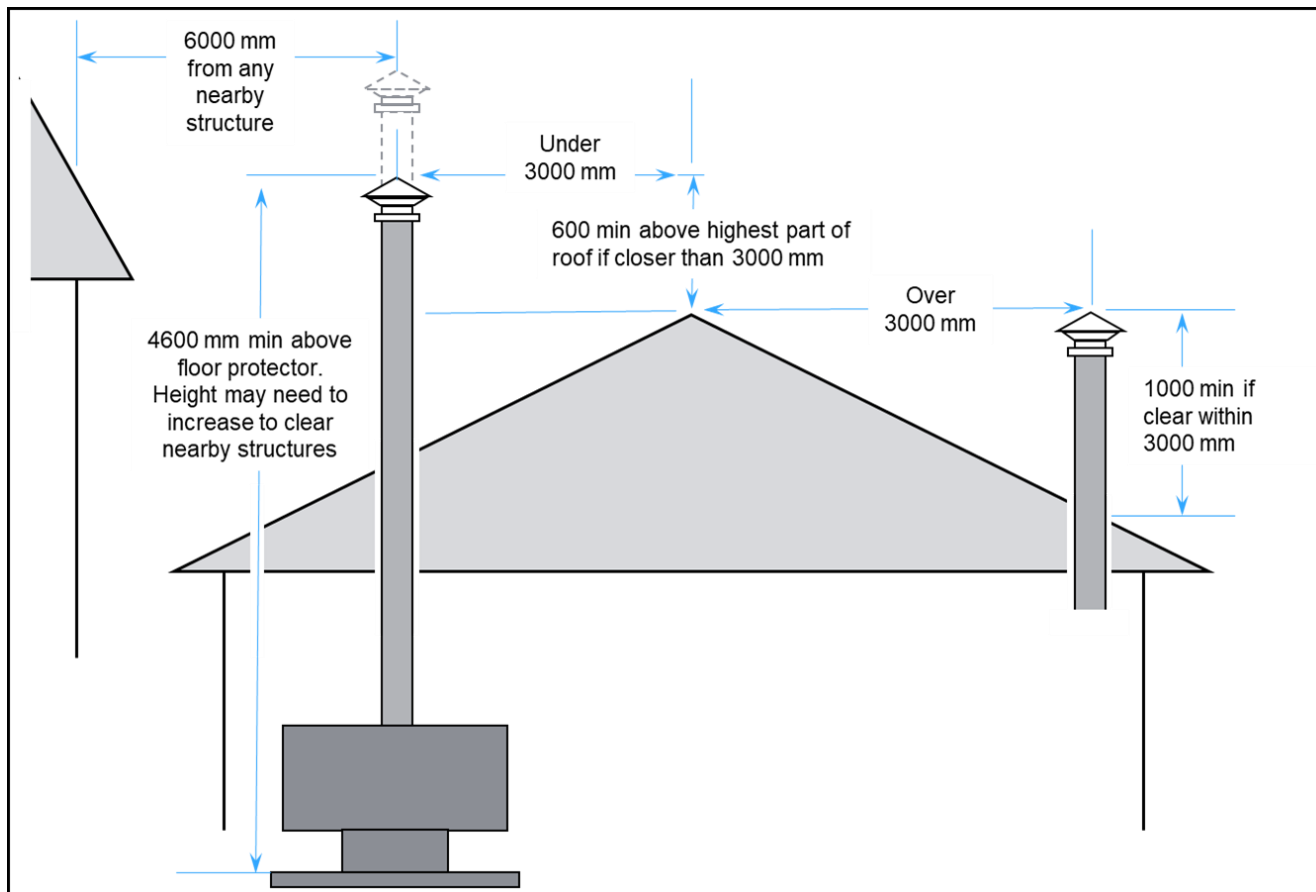
Figure 1 - A guide to flue terminations
